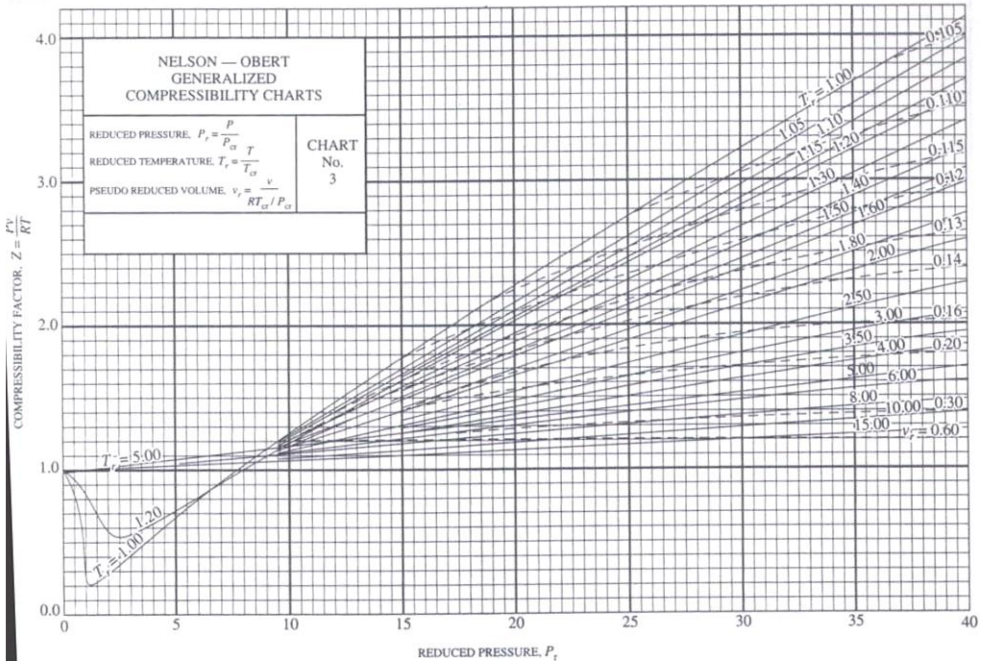
Nelson-Obert Generalized (Averaged) Compressibility Chart
